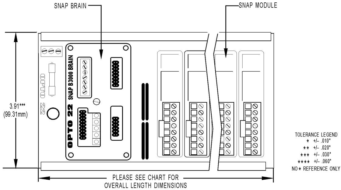
Dimensions—B-Series Racks Without Terminal Strips
