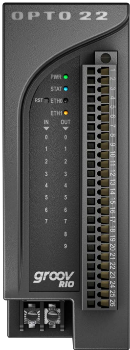
GRV-R7-MM1001-10 and GRV-R7-MM2001-10 Channel Positions
