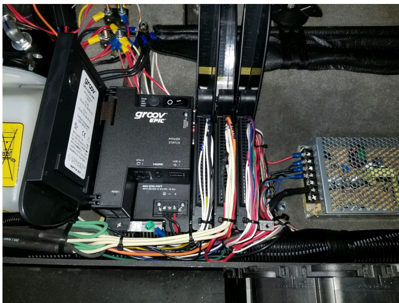
groov EPIC embedded inside the truck's lift system
